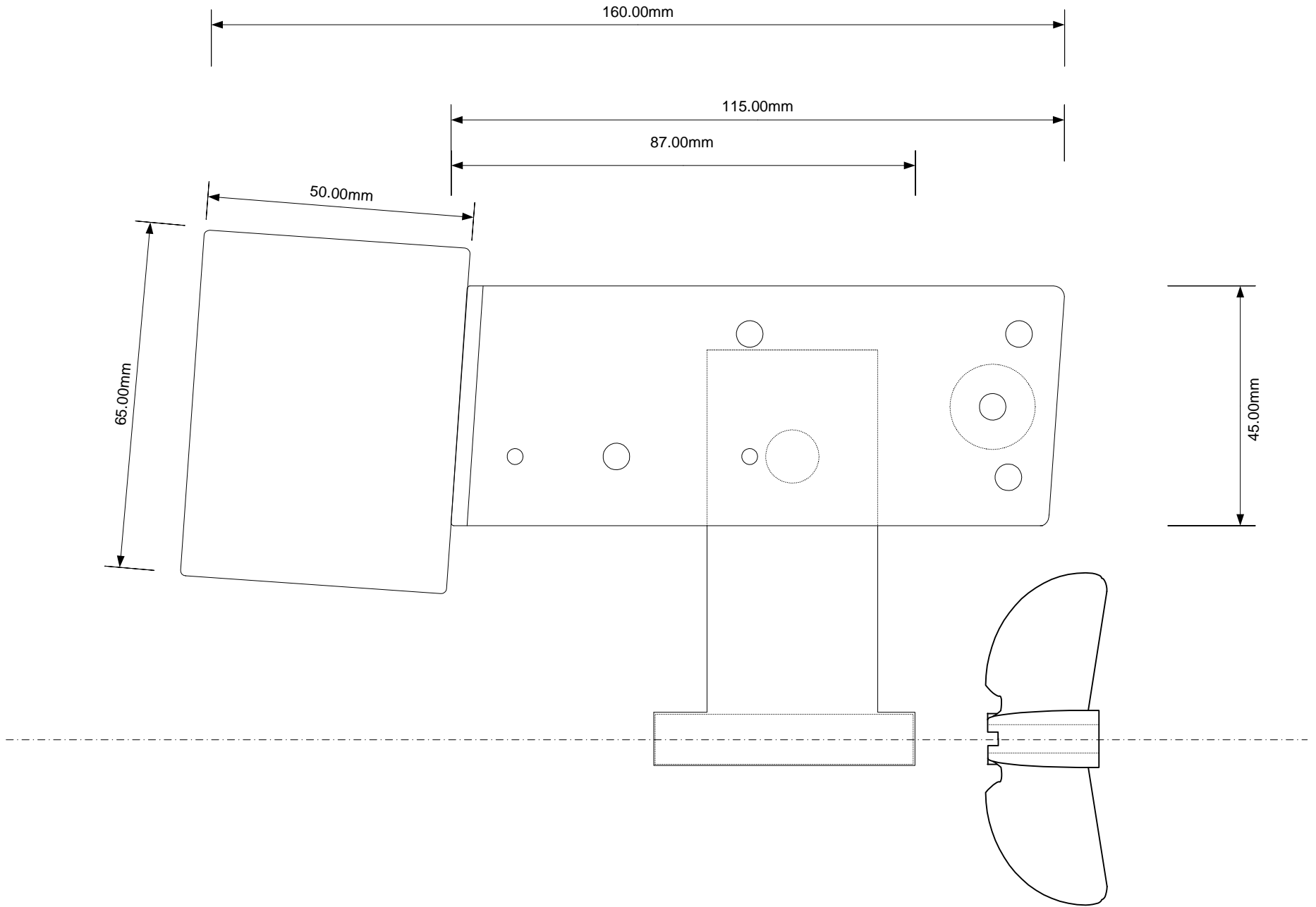
Outrigger Assembly
